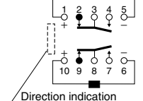
2-coil latching
